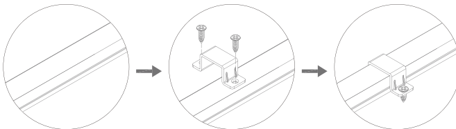
TL120NEON-TB-PCC -Polycarbonate mounting clip (one clip per foot)
