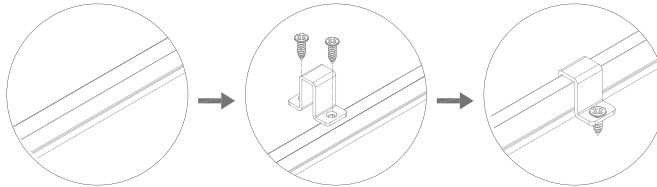
TL120NEON-SB-PCC -Polycarbonate mounting clip (one clip per foot)
